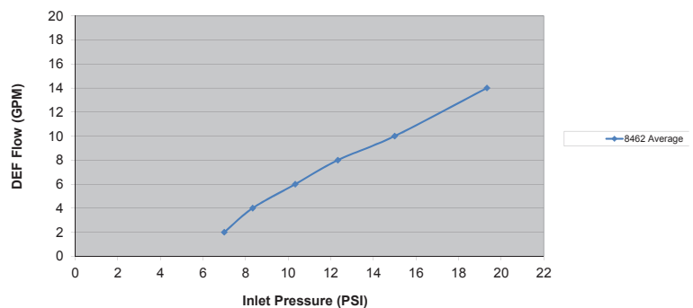
008462 DEF Plastic Nozzle Average Back Pressure Performance Verification
